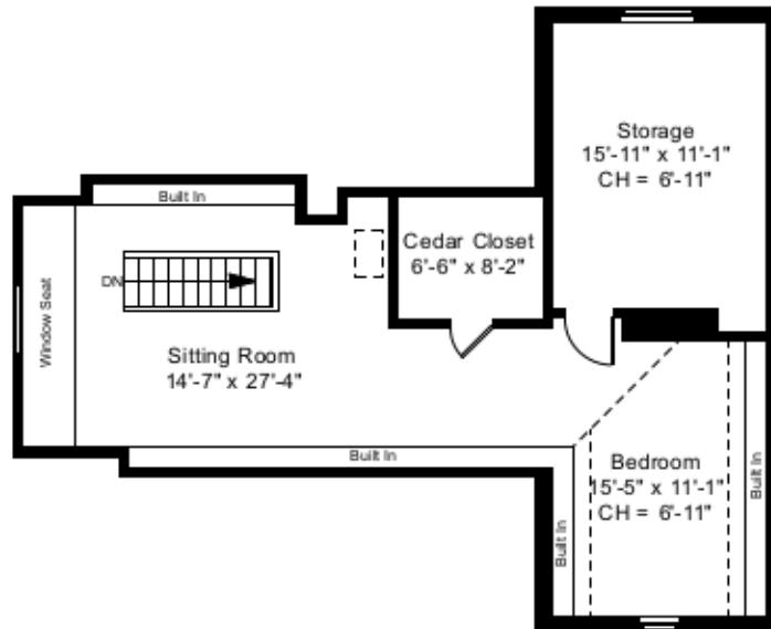
Third Floor Plan Ceiling Height = 7'-10"
