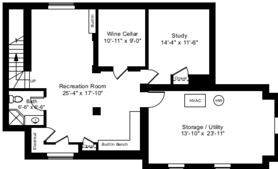
Lower Level Plan Ceiling Height = 7'-2"
