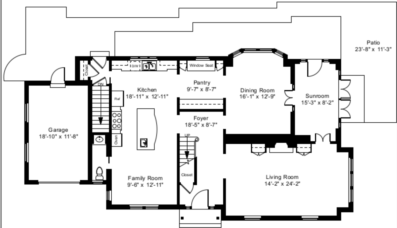
First Floor Plan Ceiling Height = 9'-0"
